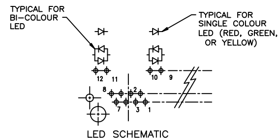
BI-COLOUR LED DETAIL (RED/YELLOW AND GREEN/ORANGE LED'S ARE ALSO AVAILABLE)
