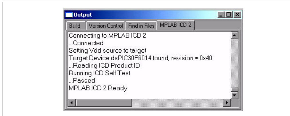
FIGURE 4-4: MPLAB ICD 2 CONNECTION MESSAGE WITH dsPIC30F6014
