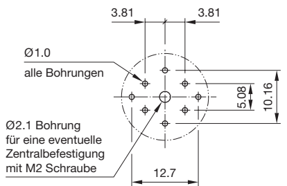
Component layout 1
