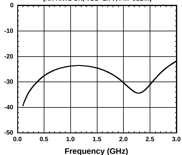
TX-ANT2 Isolation vs. frequency
