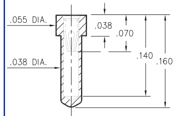
0529-0-15-XX-10-XX-10-0 .040 min. mounting hole
