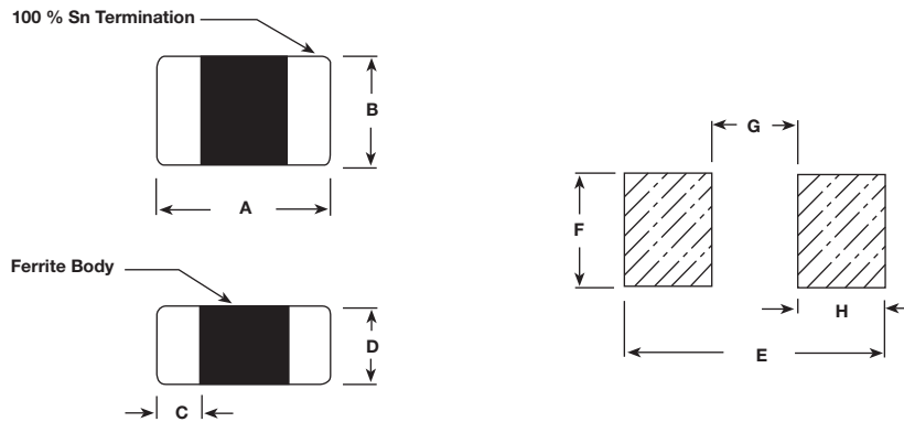
Dimensional Outline
