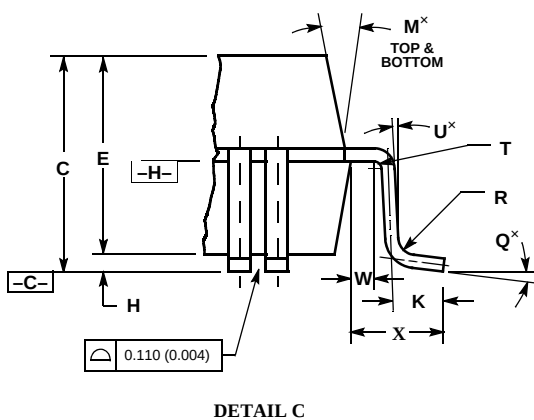
Case 864A-03 Figure 6. 160 QFP Package Dimensions
