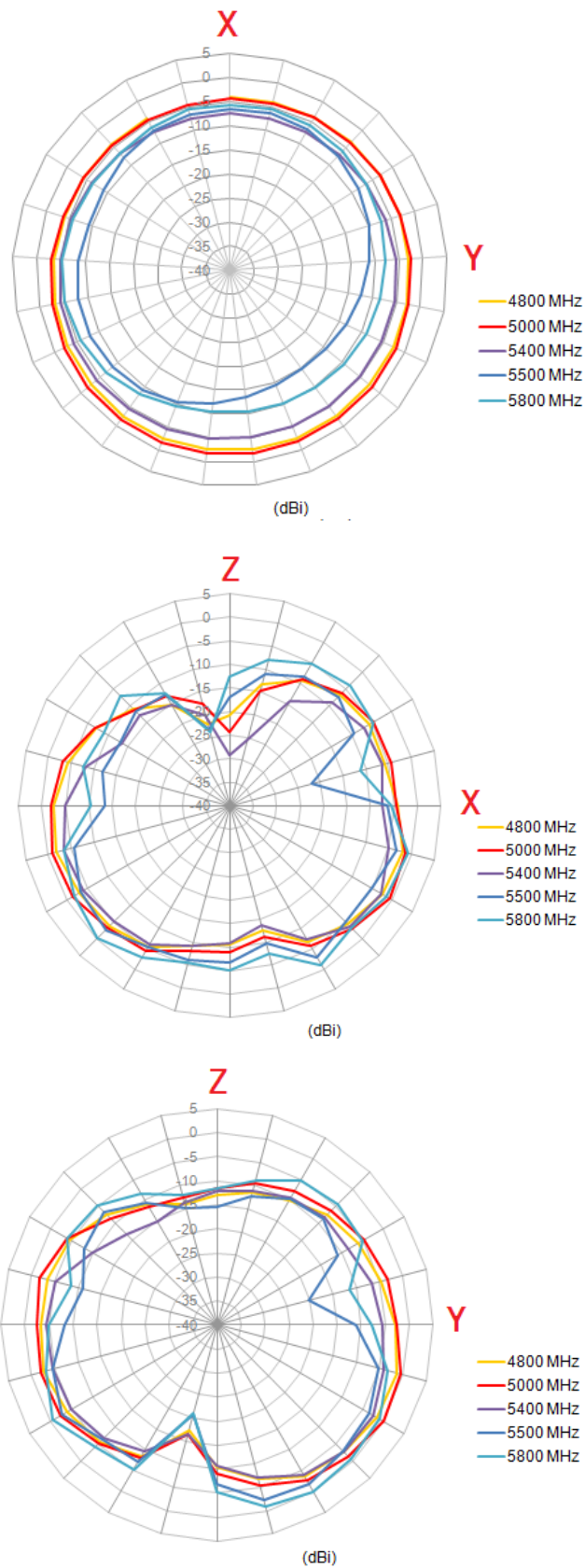
Figure 14. 2D Radiation Pattern at 5800MHz band
