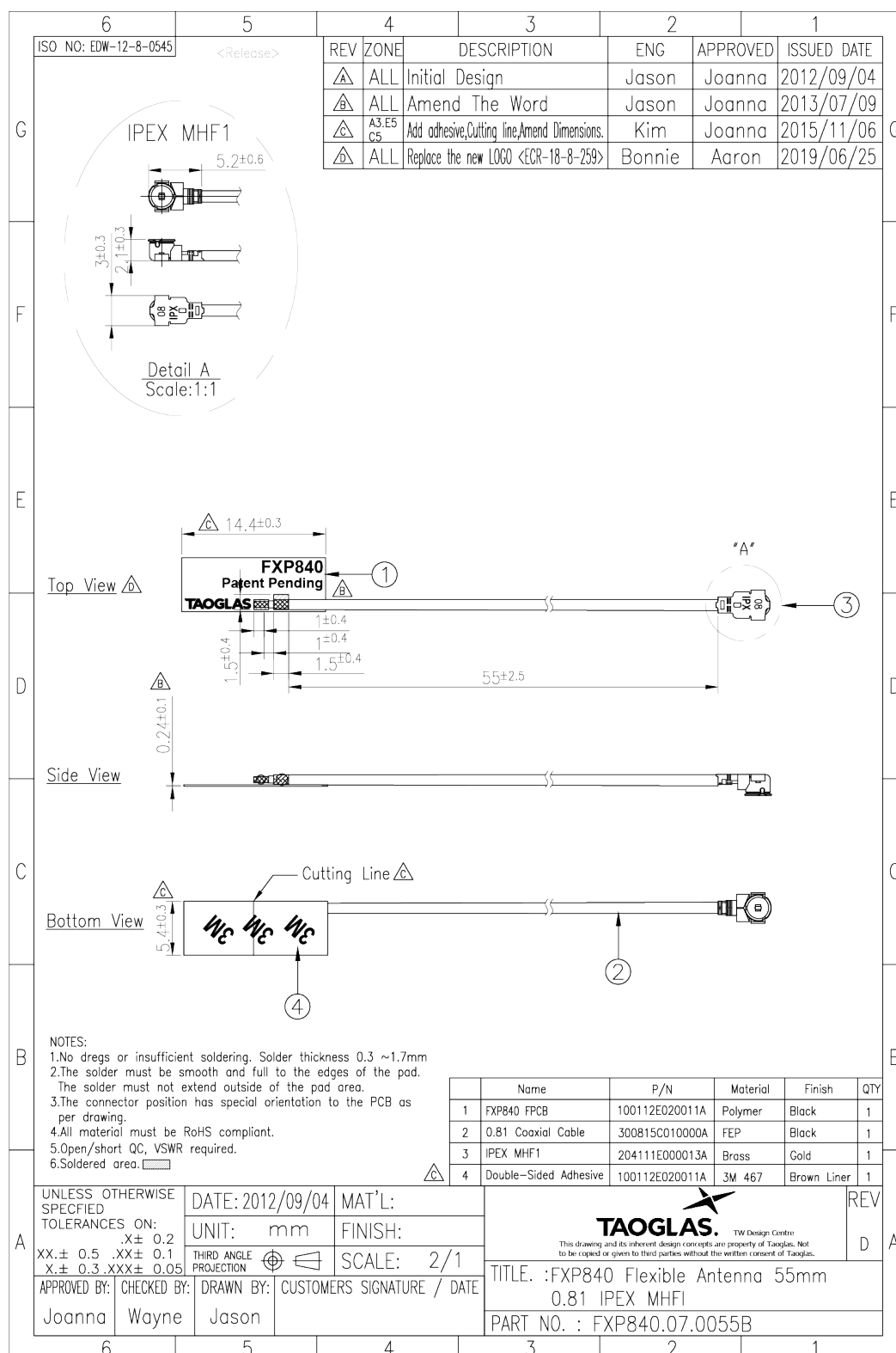
Figure 15. Antenna Drawing.
