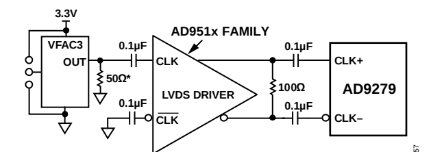
Figure 55. Differential LVDS Sample Clock
