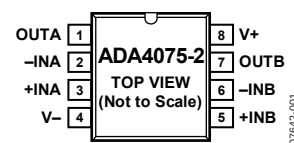
Figure 1. 8-Lead SOIC
