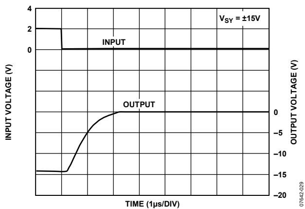
Figure 35. Negative Overload Recovery
