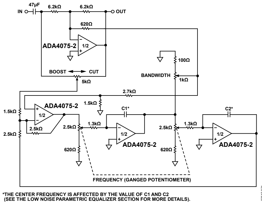
Figure 69. Low Noise Parametric Equalizer
