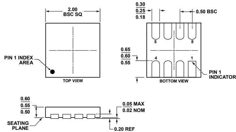
Figure 72. 8-Lead Lead Frame Chip Scale Package [LFCSP_WD] 2 mm x 2 mm Body, Very Very Thin, Dual Lead (CP-8-6)
