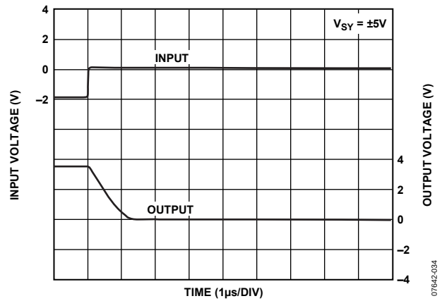
Figure 42. Positive Overload Recovery
