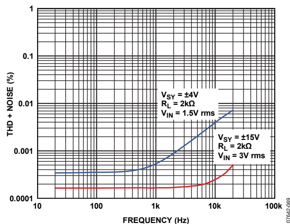
Figure 64. THD + Noise vs. Frequency
