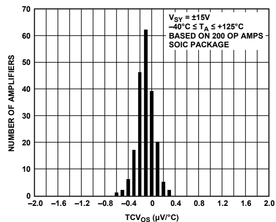
Figure 5. Input Offset Voltage Drift Distribution
