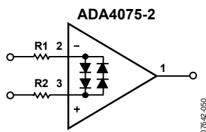
Figure 63. Input Protection
