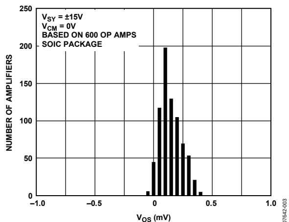
Figure 3. Input Offset Voltage Distribution
