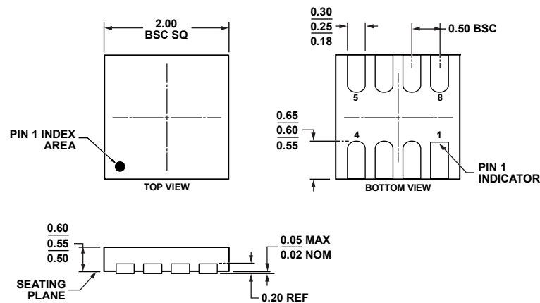
Figure 72. 8-Lead Lead Frame Chip Scale Package [LFCSP_WD]
