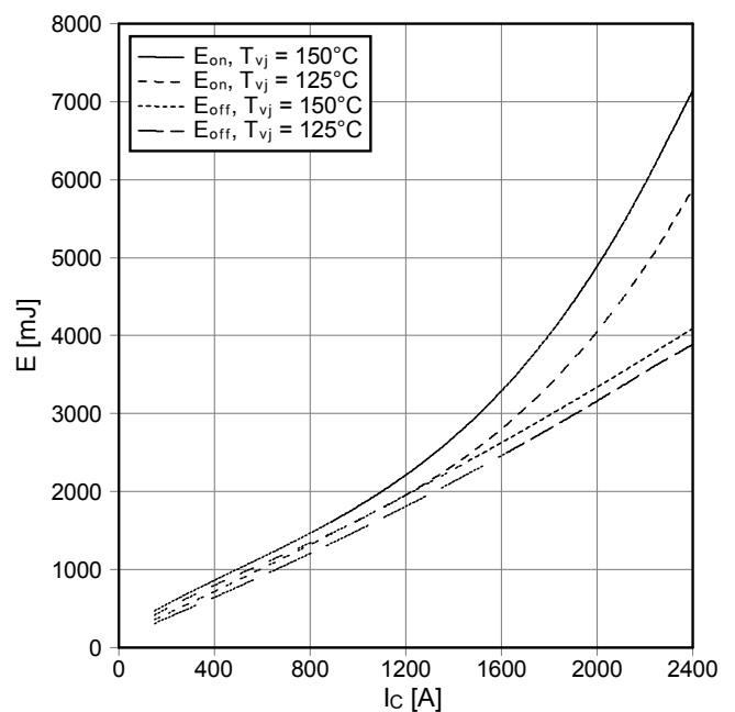
Schaltverluste IGBT-Wechselr. (typisch) switching losses IGBT-inverter (typical) E_{on} = f(I_C) , E_{off} = f(I_C) V_{GE} = \pm 15\text{ V} , R_{Gon} = 0.62\ \Omega , R_{Goff} = 2.4\ \Omega , V_{CE} = 1800\text{ V} , C_{GE} = 220\text{ nF}
