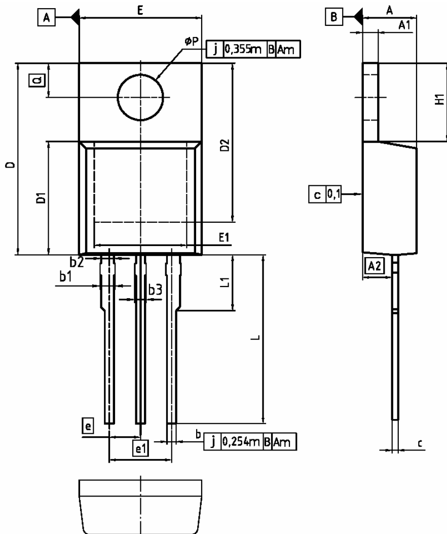
PG-TO220-3-1
