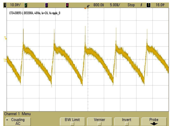
Figure 5. Typical VOUT ripple 48VIN 2A load
