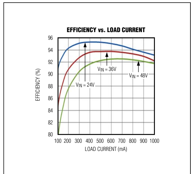
Figure 2. MAX17502G Efficiency vs. Load Current
