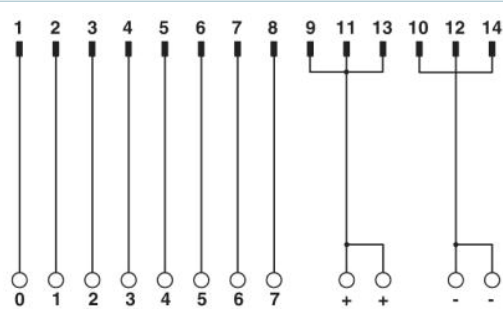
VIP-2/SC/FLK14/PLC connection scheme
