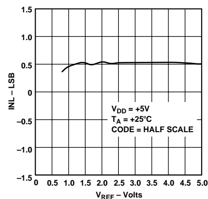
Figure 10. INL Error vs. Reference Voltage
